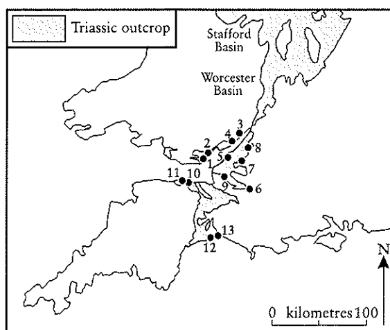
Figure 4.5 Map showing the locations of the 13 Penarth Group GCR sites: (1) Lavernock to Penarth*; (2) Stormy Down; (3) Wainlode Cliff*; (4) Westbury Garden Cliff*; (5) Aust Cliff*; (6) Hapsford Bridge; (7) Barnhill; (8) Wetmoor*; (9) Lulsgate; (10) St Audries Bay*; (11) Blue Anchor Point*; (12) Culverhole Point*; (13) Pinhay Bay. * Denotes that the site also exposes important Triassic red beds.
