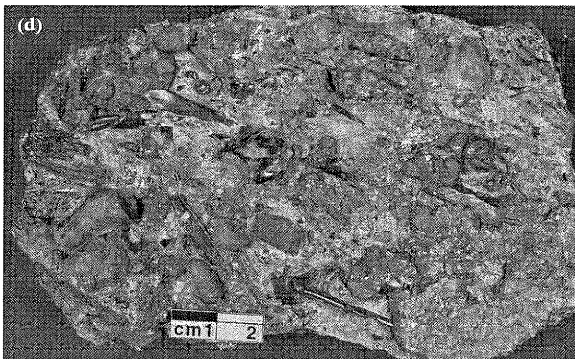
Figure 4.4 – contd. (d) Cut section through the basal 'Rhaetic bone beds' from Westbury Garden Cliff. The surface shows numerous well-preserved elongate bones of the small reptile Pachystrophia , showing weak current alignment. Other clasts include coprolites (e.g. immediately above the scale bar), some larger, abraded, bone fragments (far left, middle) and inorganic phosphate nodules. White patches of crystalline pyrite occur in association with the bones; the matrix is 70% disseminated pyrite. (Photo courtesy C.N. Trueman)
