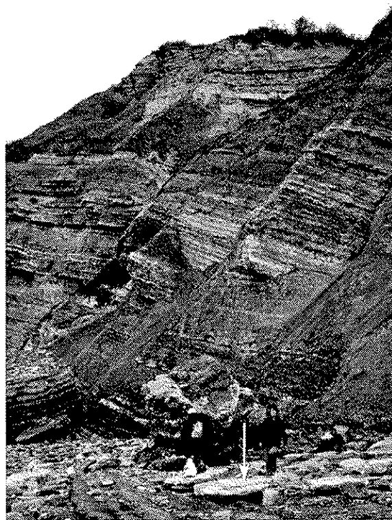
Figure 4.24 Detail of the multiple faults at Blue Anchor Point, disturbing the succession of Blue Anchor Formation (lower part of cliff) overlain by Westbury Formation at the top. A boulder of the latter, with the bone bed (arrowed), lies on the beach. (Photo: K. A. Kermack.)
