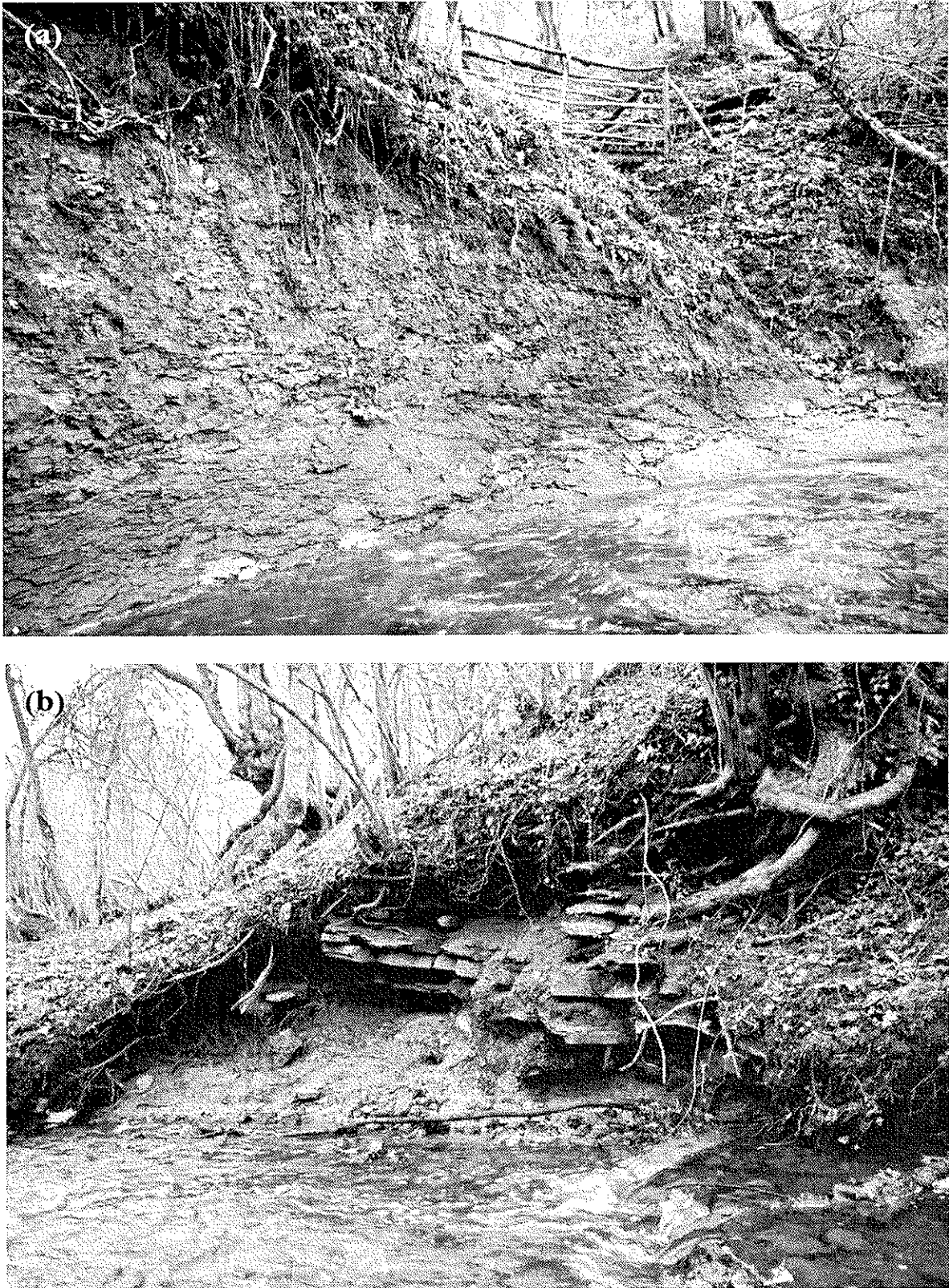
Figure 4.19 Wetmoor stream sections showing small exposures of Triassic sediments. (a) Mercia Mudstone Group mudstones, seen in the northern end of the western GCR area; (b) Cotham Member limestones and clays, and the Cotham Marble, which are overlain by basal Lias units, in the eastern GCR area. (Photos: R. Cottle.)
