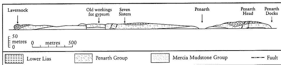
Figure 4.6 Section of the cliffs from Lavernock to Penarth, showing the occurrence of the Mercia Mudstone, Penarth, and Lias groups. (After Woodward, 1888.)
